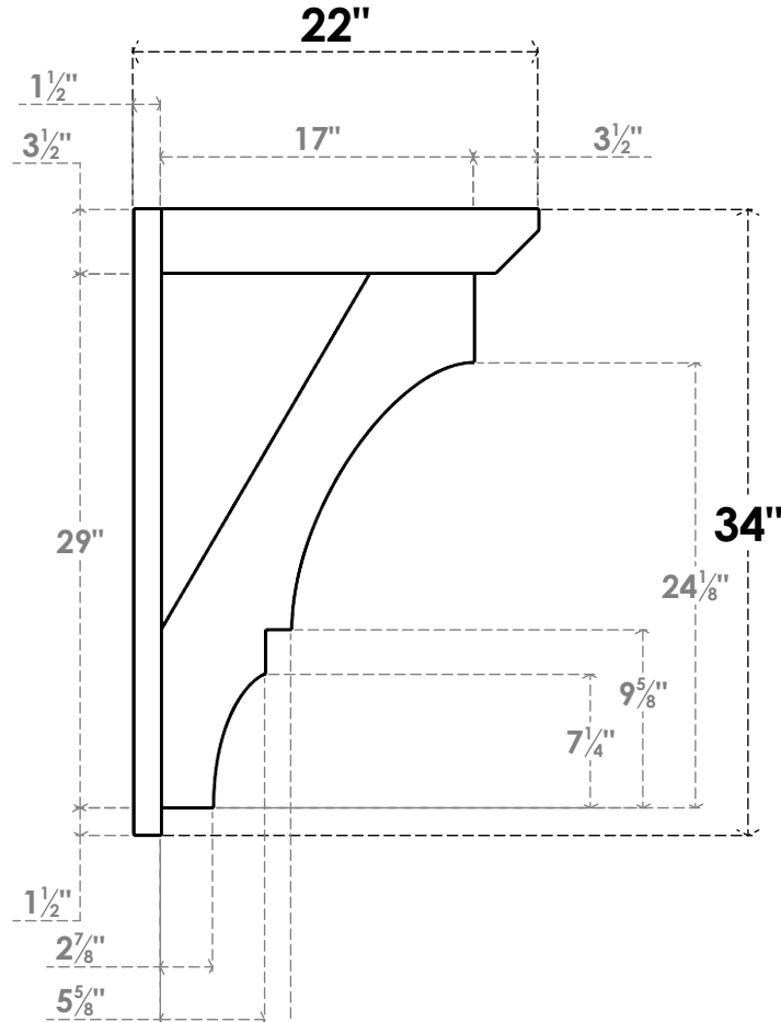
SIDE PROFILE
